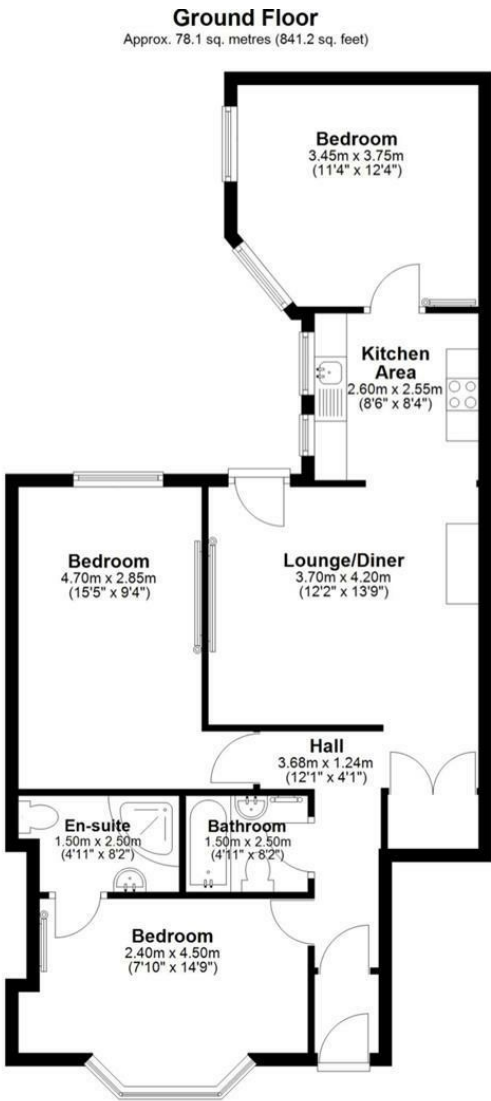
Total area: approx. 78.1 sq. metres (841.2 sq. feet)
